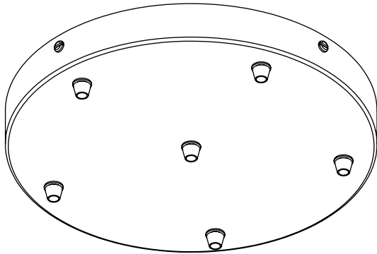
6-drop - 250mm Dia
