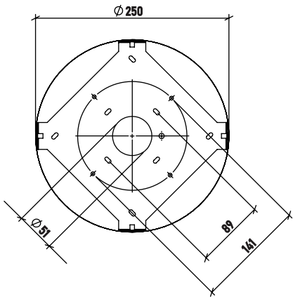
250 dia Canopy - Liner
