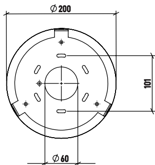
200 dia Canopy - Liner
